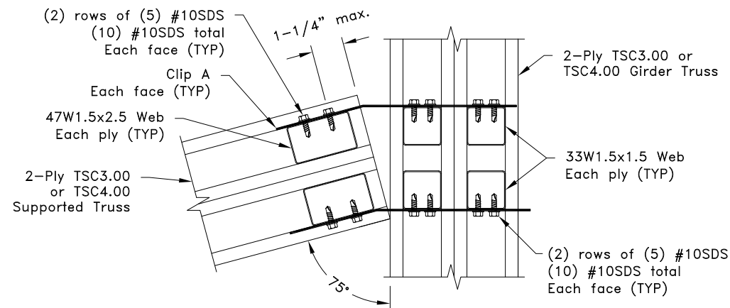
Web Connection Plan View
