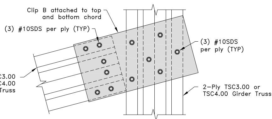
Chord Connection Plan View
